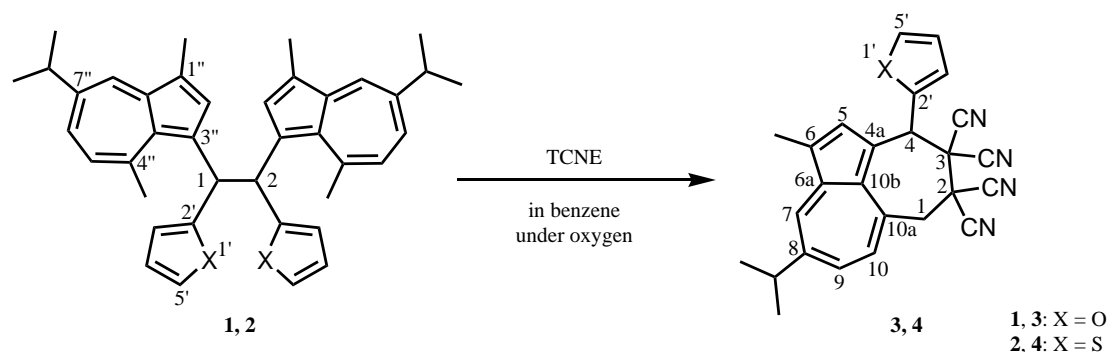
Figure 3. The reactions of the title meso forms 1 and 2 with a two molar amount of TCNE in benzene at 25 °C for 5 h (for 1 ) and 48 h (for 2 ) under oxygen.
