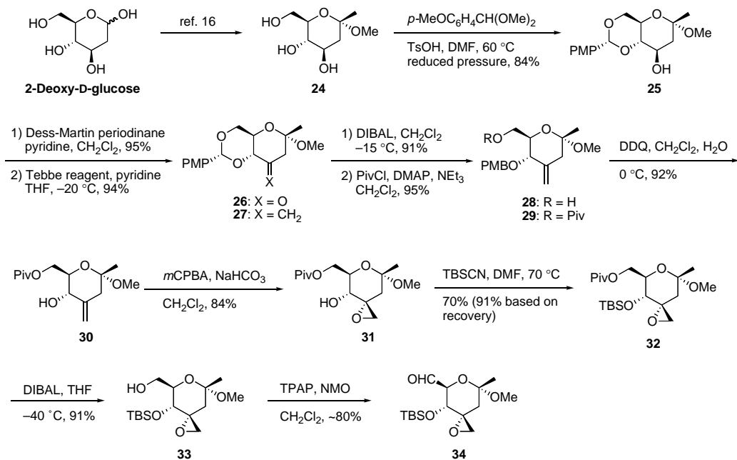
Scheme 5. Synthesis of segment C.
