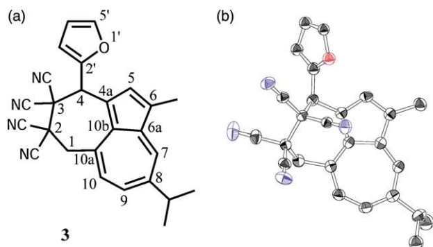
Figure 4. (a) The molecular structure of 3 . (b) The ORTEP drawing of 3 (30% probability thermal ellipsoids).
