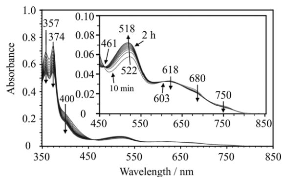
Figure 5. The time-dependent visible spectra for the reaction of 1 (2.0 mg, 3.6 \mu\text{mol} ) with TCNE (1.0 mg, 7.8 \mu\text{mol} ) in benzene (10 mL) at 25 °C for 2 h under argon. Length of the cell: 0.1 cm. Interval time: 10 min. \lambda_{\text{max}} 357, 374 and 400sh nm: the specific bands based on TCNE; \lambda_{\text{max}} 518 nm: the specific band based on the formation of the CT complex \mathbf{a}_1 (see Scheme 1) (the time to reach maximum absorption = 2 h); \lambda_{\text{max}} 618, 680sh and 750sh nm: the specific bands based on 1 .
