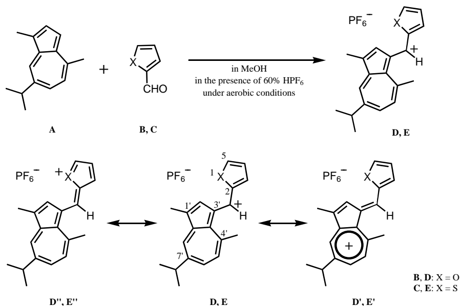
Figure 1. The reactions of A with B and C in \text{CH}_3\text{OH} with \text{HPF}_6 under aerobic conditions, affording the corresponding monocation products D and E with the resonance forms of D' , E' and D'' , E'' , respectively. 10
