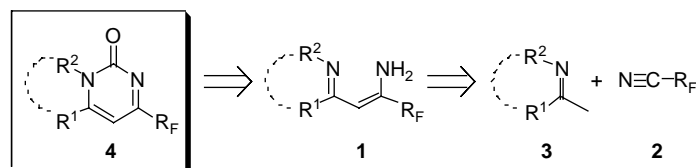
Scheme 1. Retrosynthetic analysis for compounds 1 and 4 .
