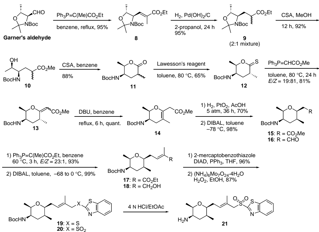
Scheme 3. Synthesis of segment B.
