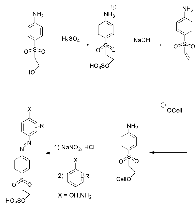
Scheme 2. Direct parallel synthesis onto cellulose.
