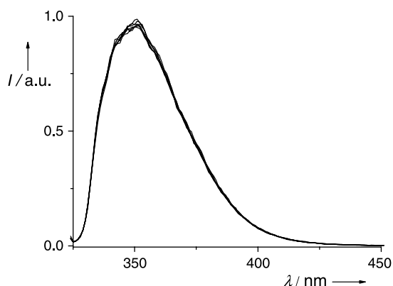
Figure 3. Fluorescence spectra ( \lambda_{\text{exc}}=320 nm) of 1 , 2.5 \times 10^{-5} M in acetonitrile upon addition of dry acetone at different concentrations ( 0 – 7.50 \times 10^{-2} M).
