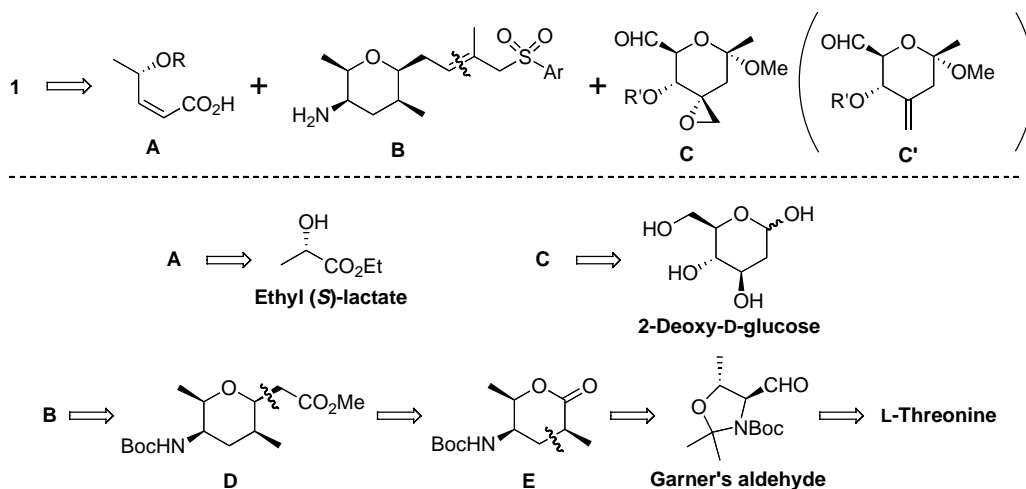
Scheme 1. Synthetic plan for FR901464.
