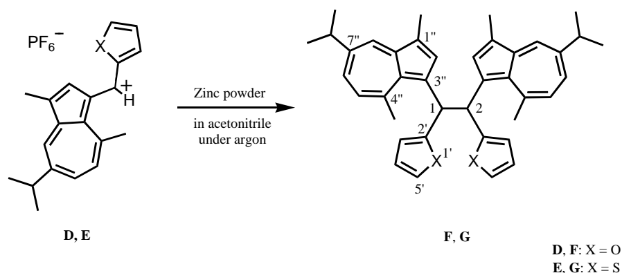
Figure 2. The reductions of D and E with zinc powder in acetonitrile at 25 °C under argon, affording a mixture of a meso form and two enantiomeric forms of the molecular structures F and G , respectively. 10
