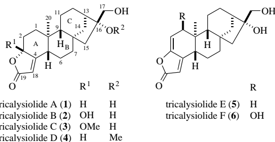
Figure 1. Structures of tricalysiolides A–F (1–6).
