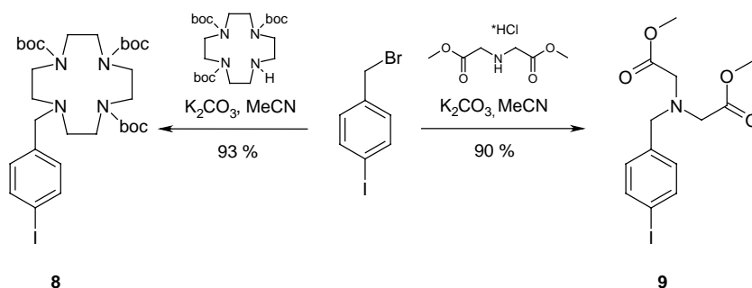
Scheme 3. Synthesis of aryl iodides 8 and 9 .
