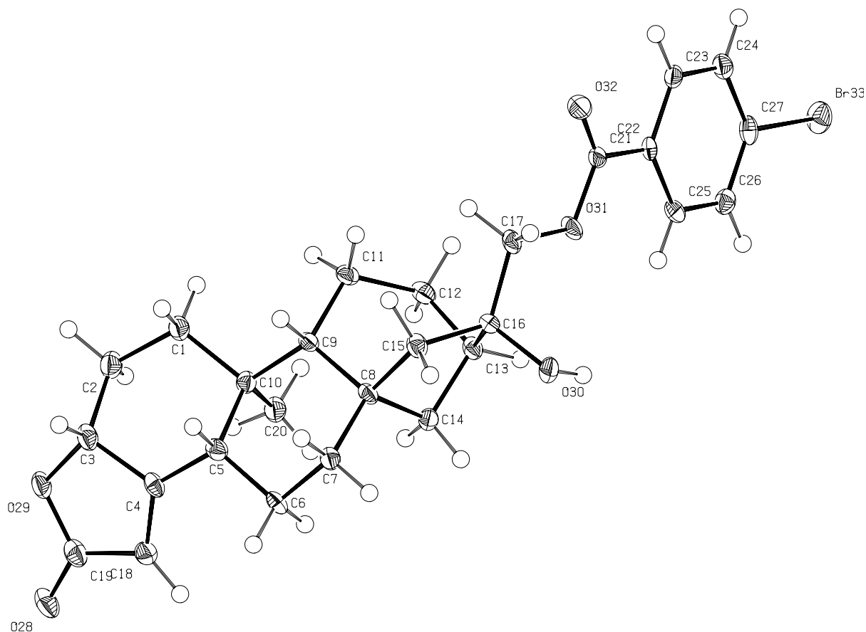
Figure 4. ORTEP representation of 7 as determined by single-crystal X-ray analysis.
