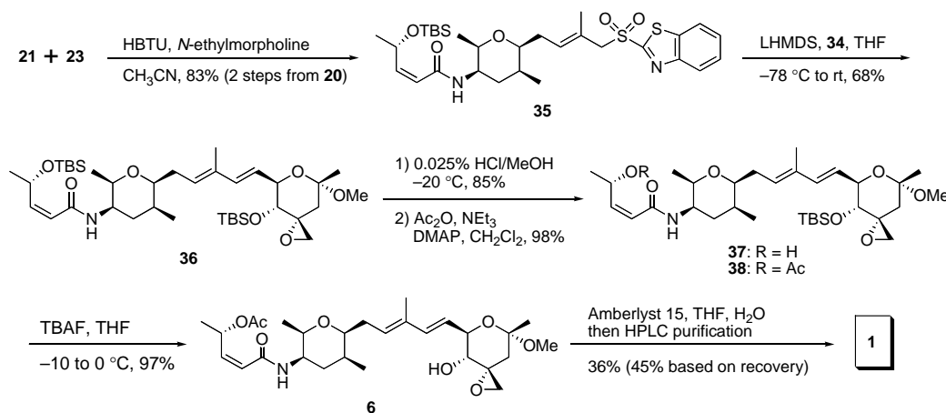
Scheme 6. Completion of the synthesis of FR901464.
