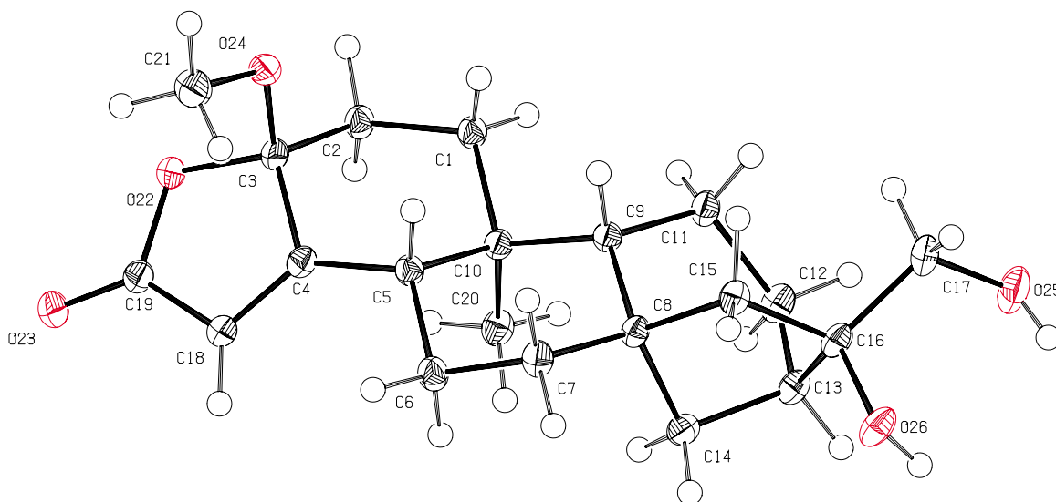
Figure 5. ORTEP representation of tricalysiolide C ( 3 ) as determined by single-crystal X-ray analysis.
