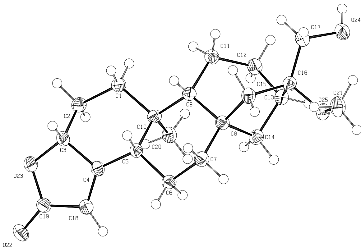
Figure 6. ORTEP representation of tricalysiolide D ( 4 ) as determined by single-crystal X-ray analysis.
