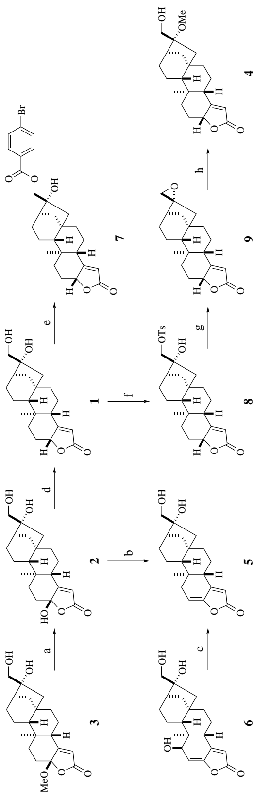
Scheme 1. Reagents and conditions: (a) LiOH, THF–H 2 O, 48 h, 87%; (b) (trimethylsilyl)diazomethane, CHCl 3 –MeOH, 1 h, 15%; (c) triethylsilane, BF 3 ·OEt 2 , CH 2 Cl 2 , 4 h, 36%; (d) NaBH 4 , EtOH, 5 min, 36%; (e) p -bromobenzoyl chloride, DMAP, pyridine–CH 2 Cl 2 , 4 h, 94%; (f) TsCl, pyridine, 18 h, 75%; (g) Na 2 CO 3 , EtOH, 48 h, 74%; (h) BF 3 ·OEt 2 , MeOH, 20 min, 31%.
