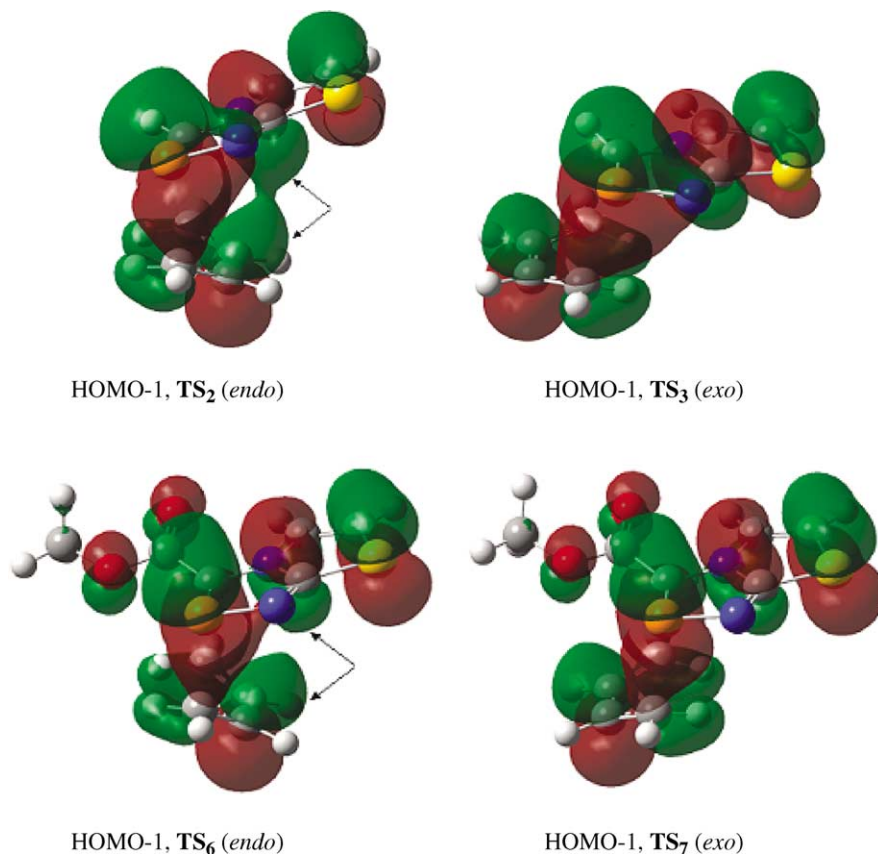
Figure 3. Secondary molecular orbital interactions in endo transition structures for DA reactions of thiazolo[3,2- d ][1,4,2]diazaphospholes ( 2 ) with 1,3-butadiene.
