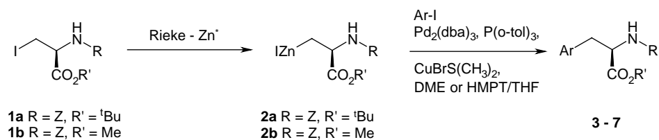
Scheme 2. Preparation of the organozinc reagents 2a and 2b and their coupling with aryl iodides.
