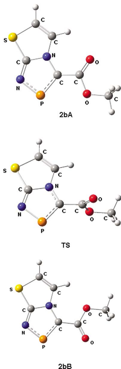
Figure 2. Optimized geometries (B3LYP/6-311G**) of the two conformers of 2b and the corresponding TS.
