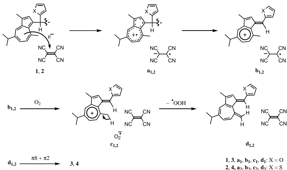
Scheme 1. A plausible reaction pathway for the formation of 3 and 4 yielded by the reactions of the title meso forms 1 and 2 with a two molar amount of TCNE in benzene at 25 °C for 5 h (for 1 ) and 48 h (for 2 ) under oxygen. The partial structures 1 , 2 and a 1,2 are illustrated.
