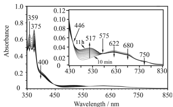
Figure 6. The time-dependent visible spectra for the reaction of 2 (2.0 mg, 3.4 \mu\text{mol} ) with TCNE (1.0 mg, 7.8 \mu\text{mol} ) in benzene (10 mL) at 25 °C for 11 h under argon. Length of the cell: 0.1 cm. Interval time: 1 h. \lambda_{\text{max}} 359, 375 and 400sh nm: the specific bands based on TCNE; \lambda_{\text{max}} 517 nm: the specific band based on the formation of the CT complex \mathbf{a}_2 (see Scheme 1) (the time to reach maximum absorption = 11 h); \lambda_{\text{max}} 622, 680sh and 750sh nm: the specific bands based on 2 .
