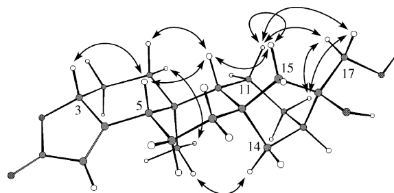
Figure 3. Selected NOESY correlations for 1 .
