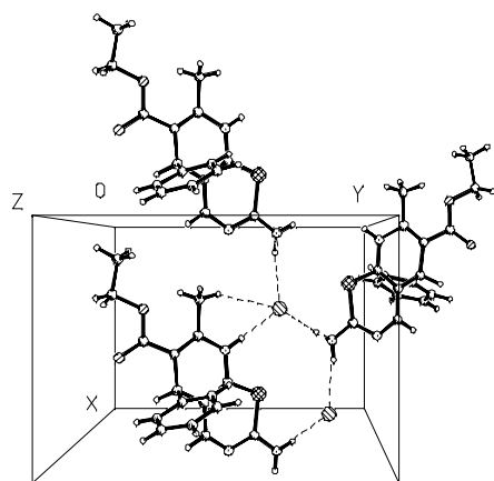
Figure 2. Projection of the molecules of 8a in the unit cell along the [001] direction and denoting the hydrogen bonds that involves the Cl atom.
