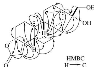
Figure 2. Selected HMBC correlations for 1 .
