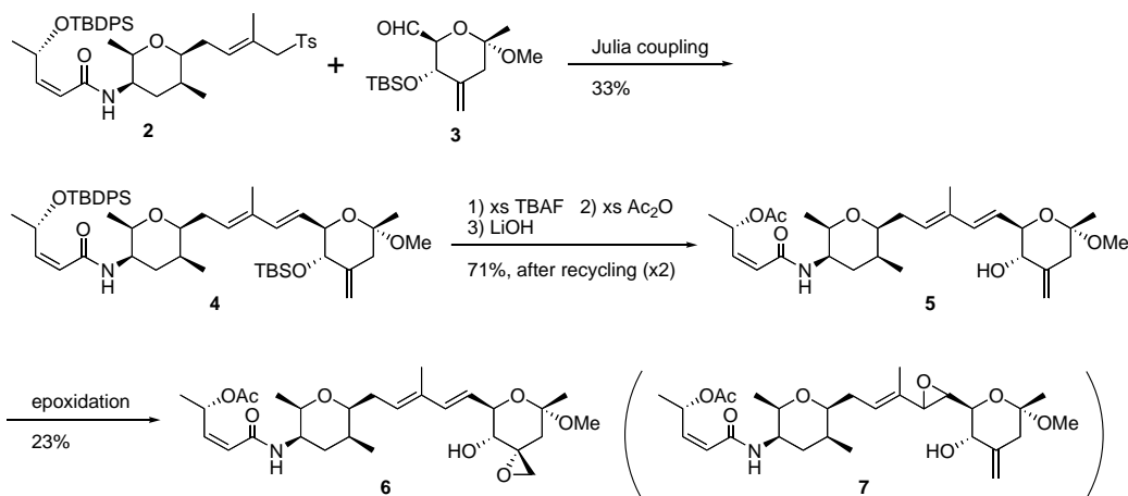
Scheme 2. Problems in our first generation synthesis.
