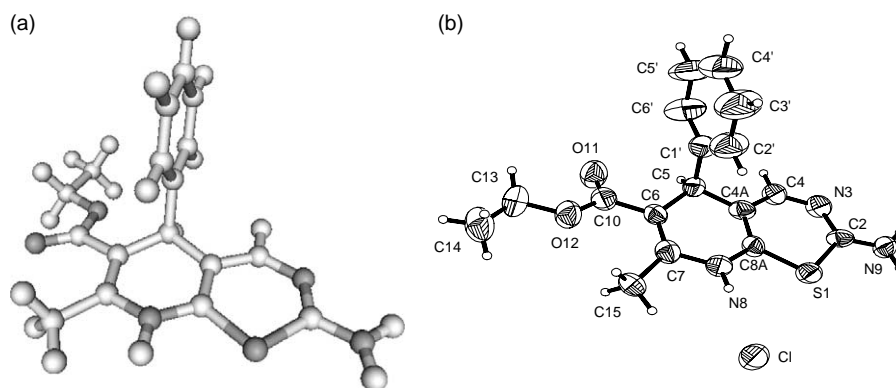
Figure 1. (a) Most stable conformation for compound 8a calculated by B3LYP/6-31G*. (b) ORTEP diagram of the crystal structure of 8a showing its atomic numbering scheme. Displacement ellipsoids are drawn at 50% probability level for non-H atoms.
