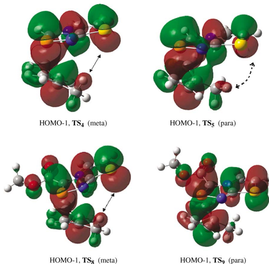
Figure 4. Secondary molecular orbital interactions in the transition structures for DA reactions of thiazolo[3,2- d ][1,4,2]diazaphospholes ( 2 ) with isoprene.
