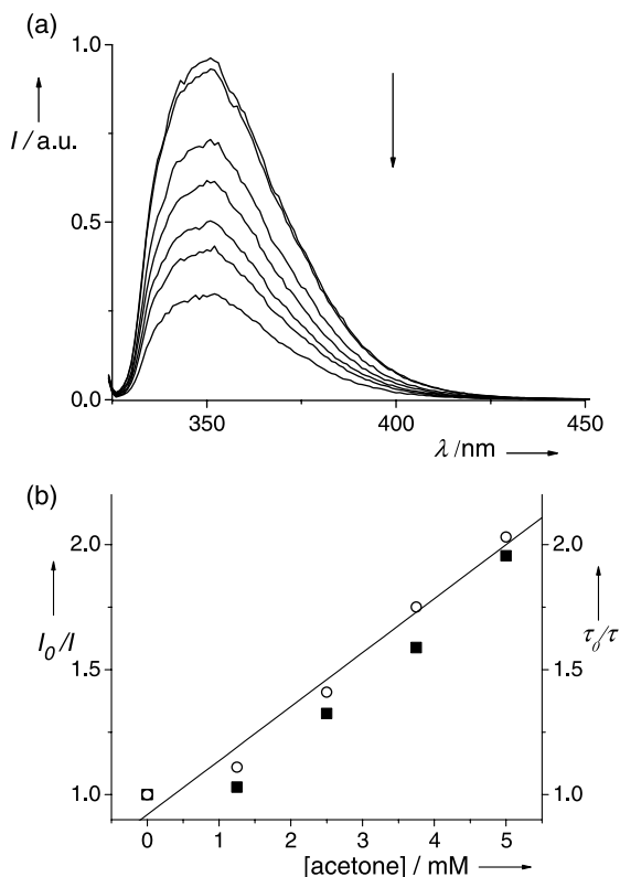
Figure 2. (a) Fluorescence spectra ( \lambda_{\text{exc}}=320 nm) of 1 , 2.5 \times 10^{-5} M in acetonitrile in the presence of increasing amounts of aqueous acetone ( 0 – 1.25 \times 10^{-2} M). (b) Stern–Volmer plot for quenching of the fluorescence of 1 by aqueous acetone, based on emission intensities (■) and lifetimes (○).
